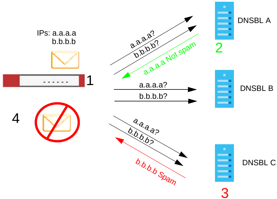
Figure 412 DNSBL Spam Detection Example
