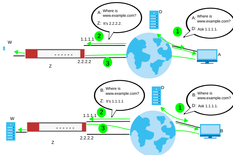
Figure 298 DNS Load Balancing Example
