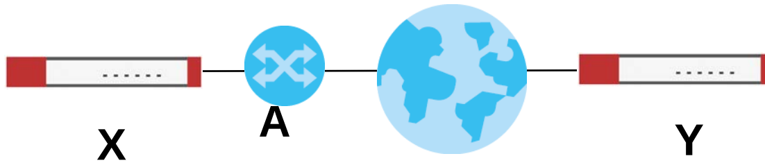
Figure 317 VPN/NAT Example
