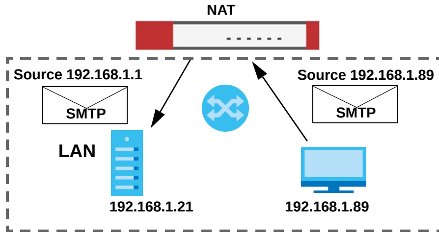
Figure 259 LAN to LAN Traffic
