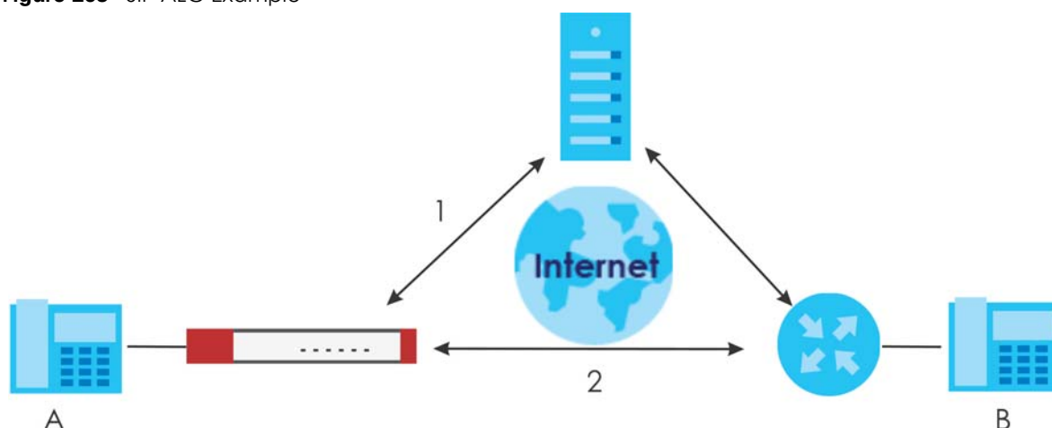
Figure 265 SIP ALG Example
