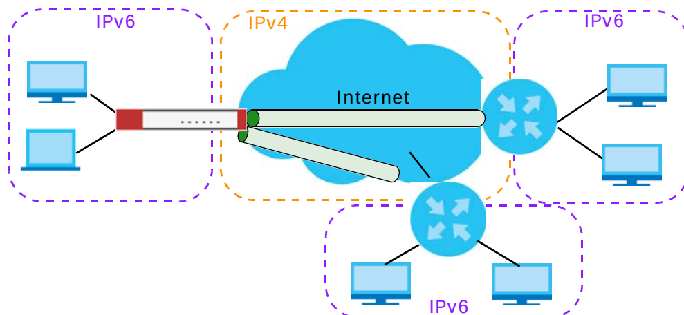
Figure 214 6to4 Tunnel
