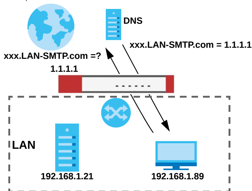
Figure 258 LAN Computer Queries a Public DNS Server
