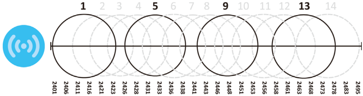
Figure 192 An Alternative Four-Channel Deployment
