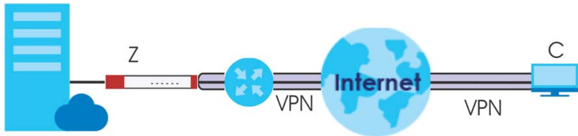
Figure 328 L2TP and Zyxel Device Behind a NAT Router
