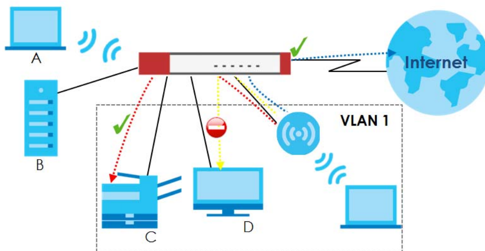
Figure 294 Layer-2 Isolation Application
