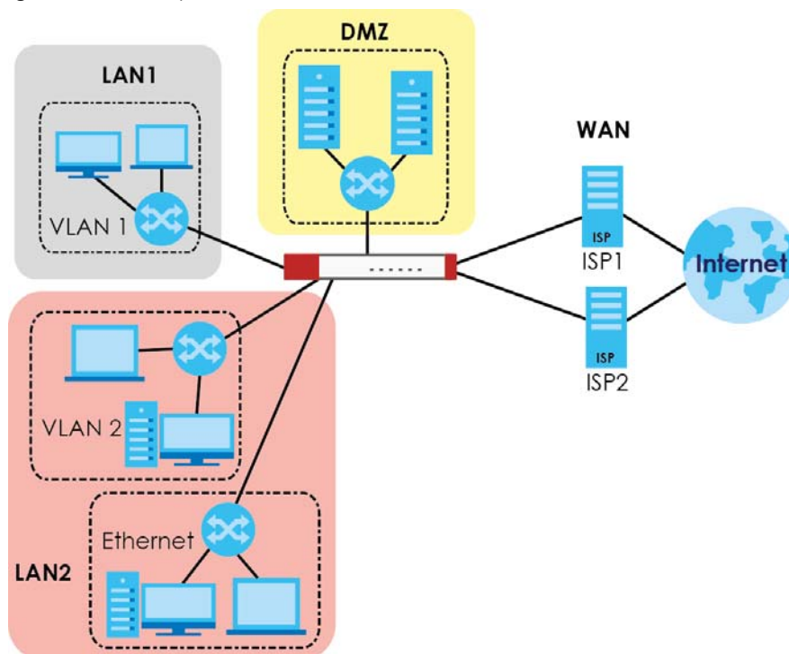
Figure 424 Example: Zones
