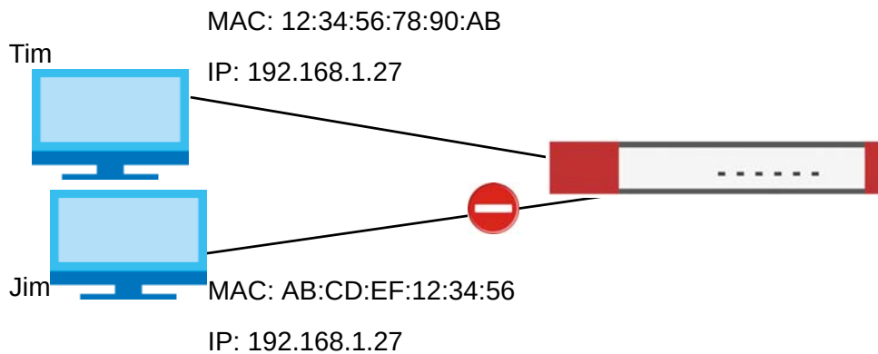
Figure 289 IP/MAC Binding Example
