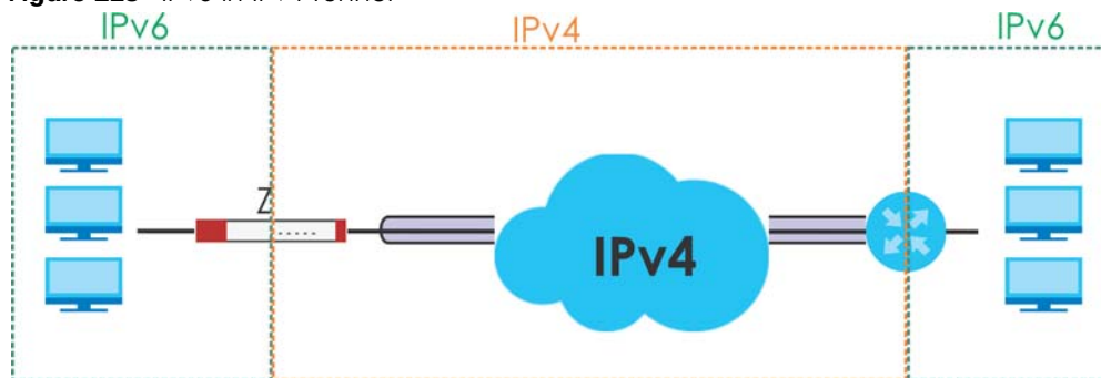
Figure 213 IPv6-in-IPv4 Tunnel
