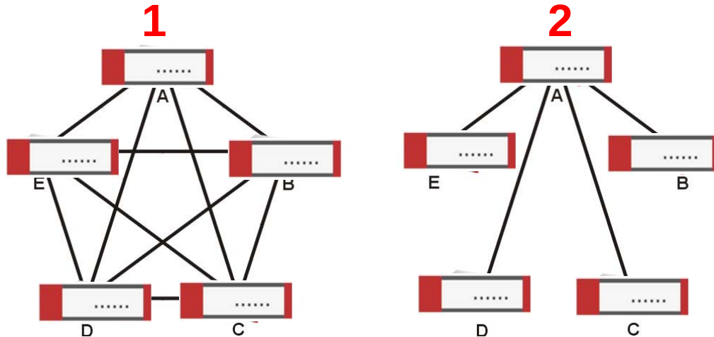
Figure 310 VPN Topologies (Fully Meshed and Hub and Spoke)
