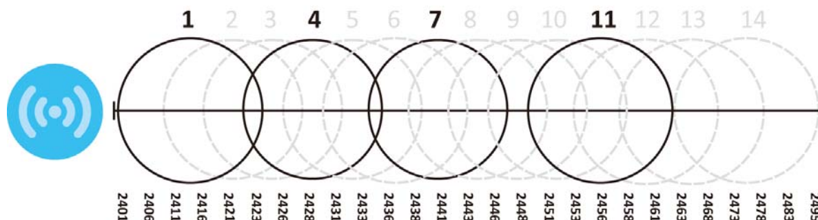
Figure 191 An Example Four-Channel Deployment
