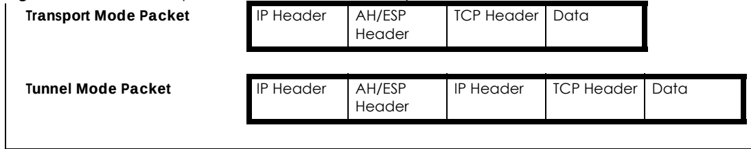
Figure 318 VPN: Transport and Tunnel Mode Encapsulation
