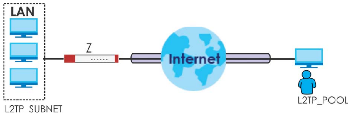
Figure 326 Policy Route for L2TP VPN
