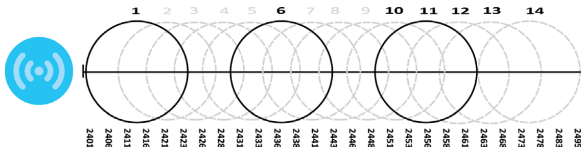
Figure 190 An Example Three-Channel Deployment
