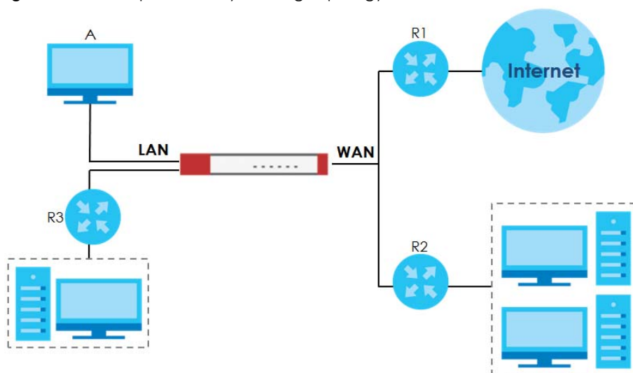
Figure 233 Example of Policy Routing Topology
