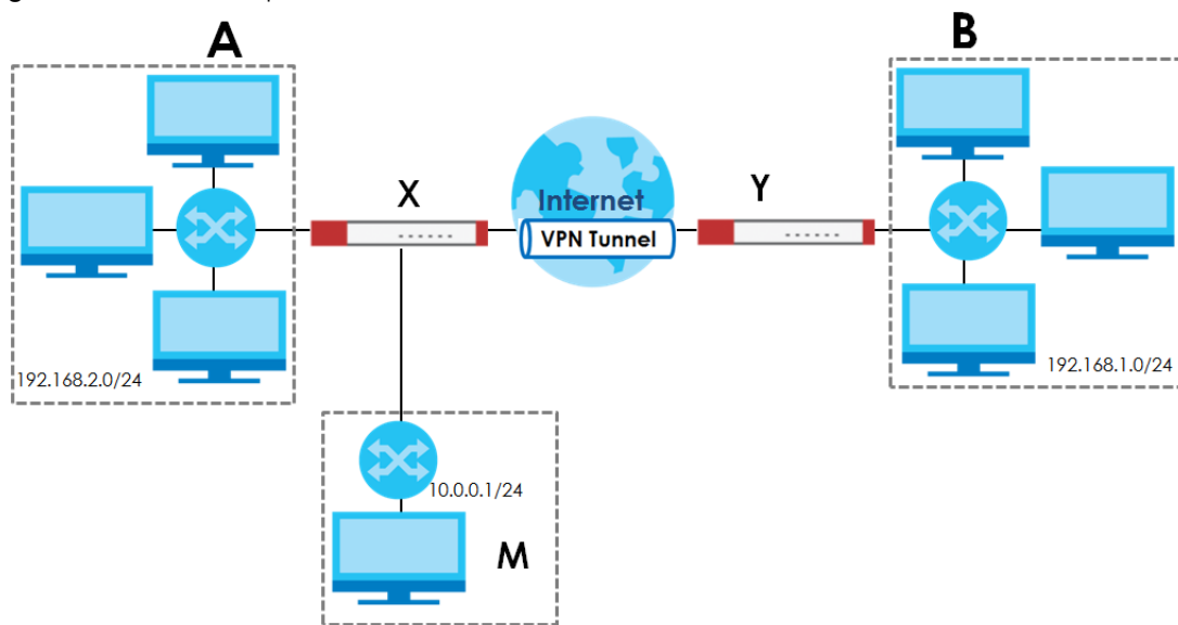
Figure 319 VPN Example: NAT for Inbound and Outbound Traffic
