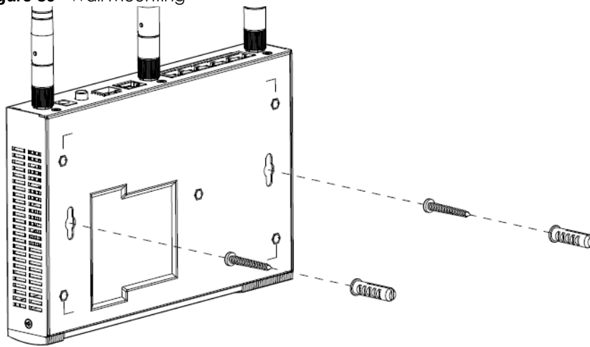
Figure 59 Wall Mounting
