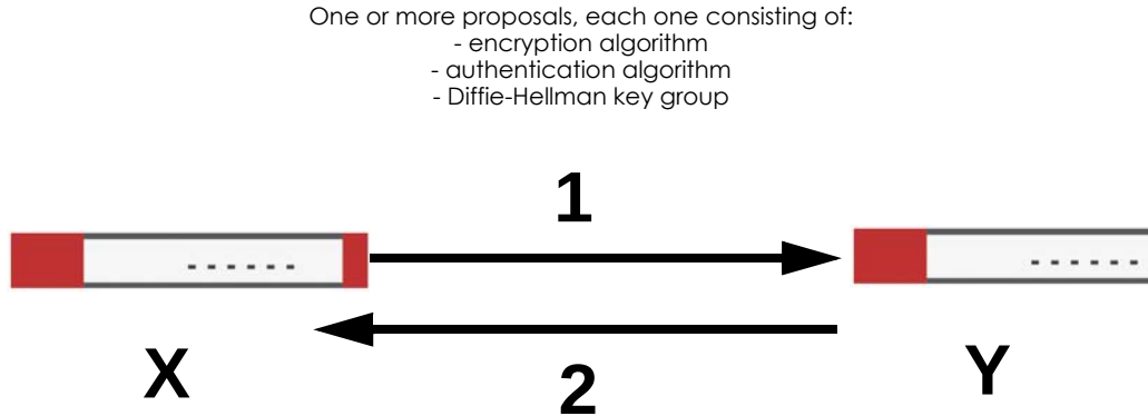
Figure 314 IKE SA: Main Negotiation Mode, Steps 1 - 2: IKE SA Proposal
