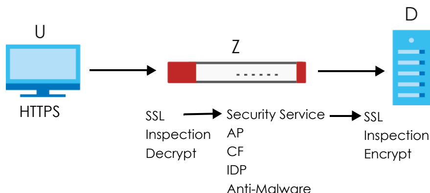
Figure 415 SSL Inspection Overview
