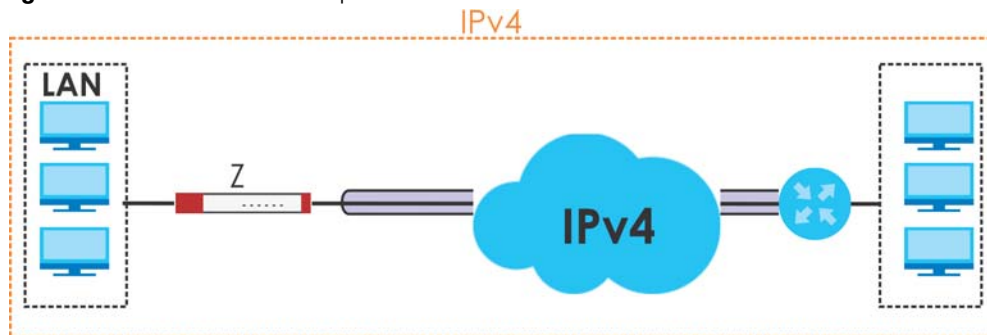
Figure 211 GRE Tunnel Example
