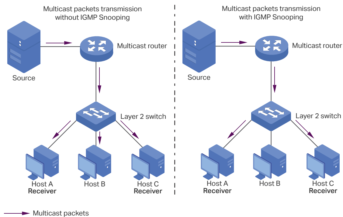
Figure 1-1 IGMP Snooping
