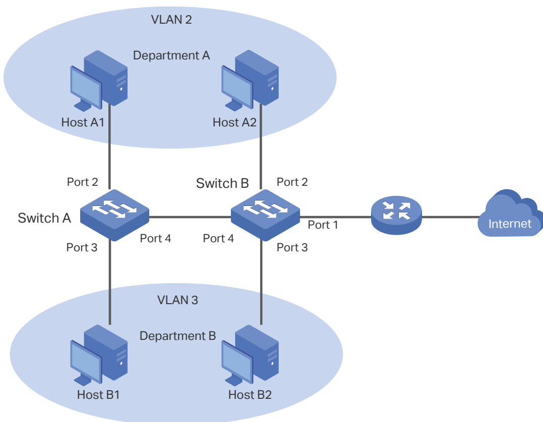
Figure 5-1 Network Topology
