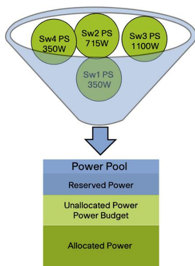
Figure 10. Redundant mode
