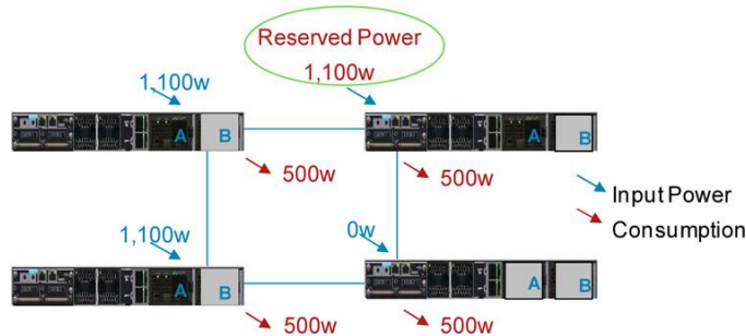
Figure 11. Redundant power
