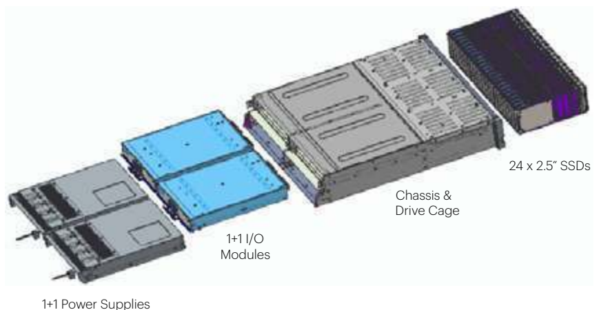
Figure 1. Platform Layout
