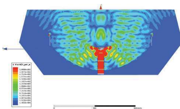
With IsoBeam
