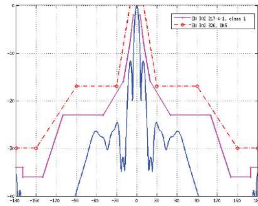
E-Plane Specs
