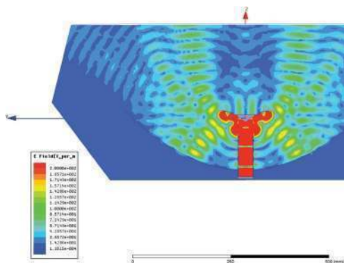
Without IsoBeam
