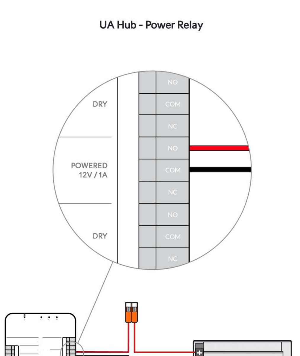
UA Hub - Power Relay
