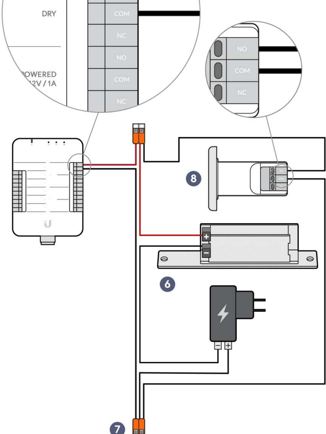
UA Hub - Dry Relay
