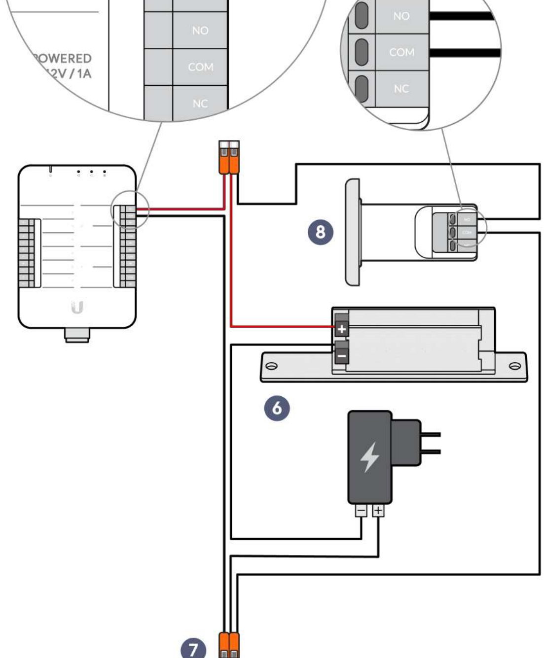
UA Hub - Dry Relay
