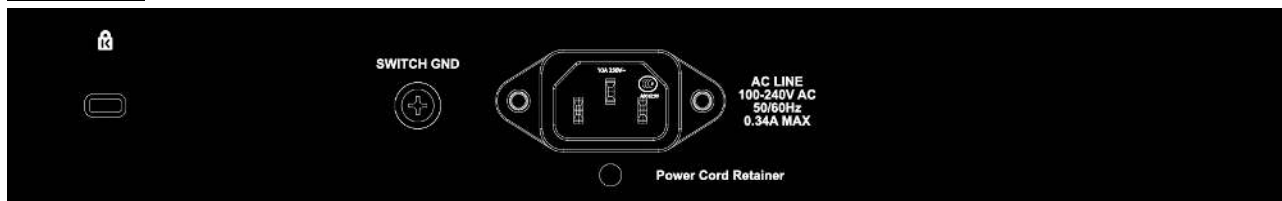
Figure 1.8 – DGS-1210-20 Rear Panel
