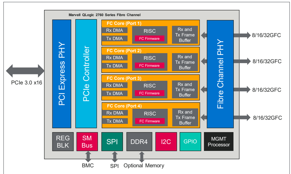
Figure 1. 2760 Series Adapter Block Diagram
