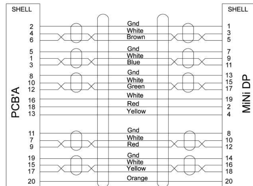
Pin Assignment
