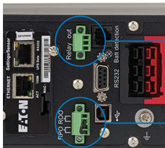
Output relay port
