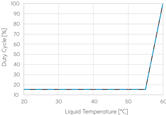
Safety Curves (PWM)
