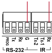
Figure 11: Connecting IR Controller
