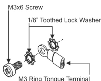
Figure 8: Grounding WP-789T , WP-789R
