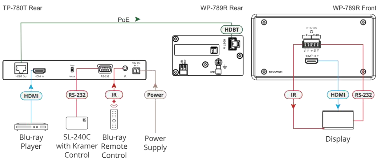
Figure 5: Connecting WP-789R to TP-780T
