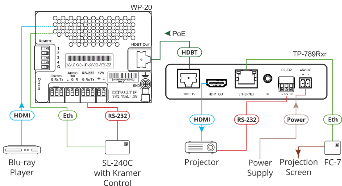
Figure 6: Connecting TP-789Rxr to WP-20
