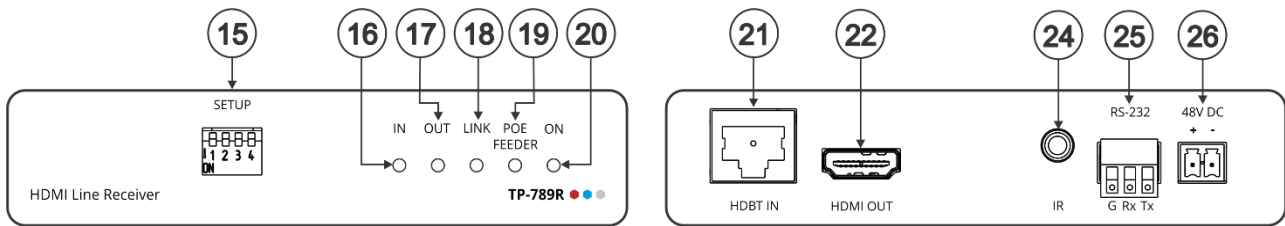
Figure 2: TP-789R
