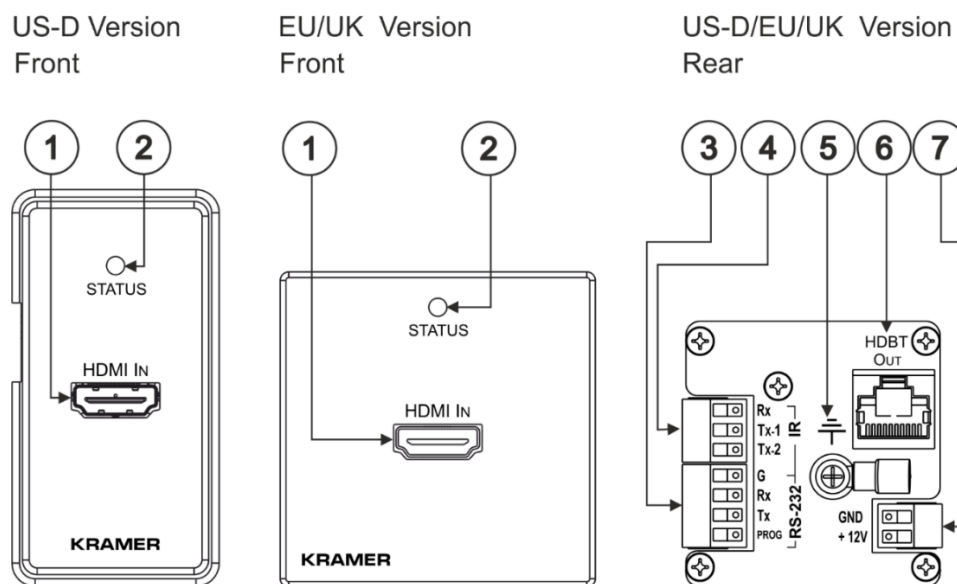
Figure 1: WP-789T
