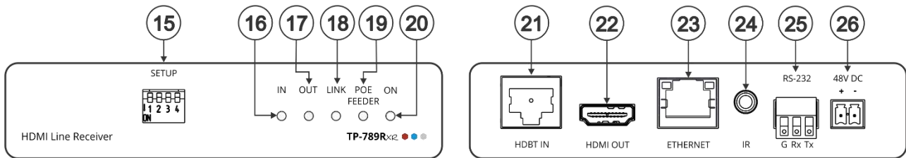
Figure 3: TP-789Rxr
