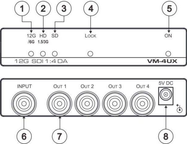
Figure 1: VM-4UX 12G SDI 1:4 DA
