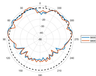
Elevation2 (Side View): 5600–5800 MHz
