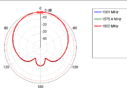
YZ Plane: 1561–1602 MHz
