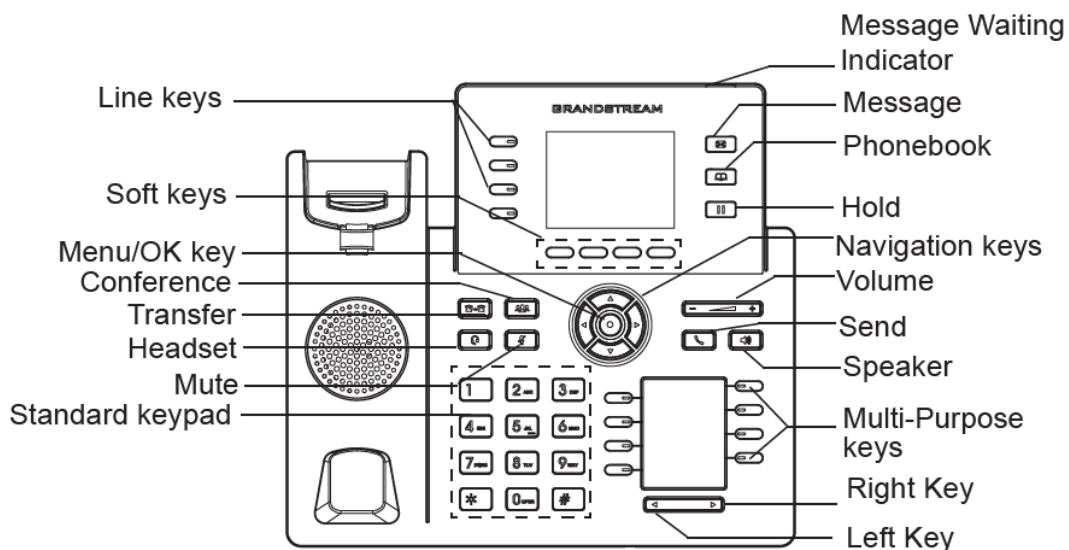
Figure 7: GRP2613 Keyboard
