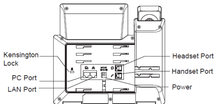
Figure 4: GRP261X/GRP2624/GRP2634 Back / Side View
