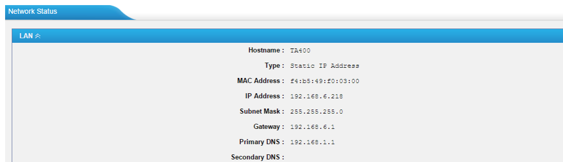
Figure 12-2 Network Status
