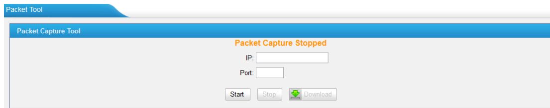
Figure 13-3 Packet Tool
