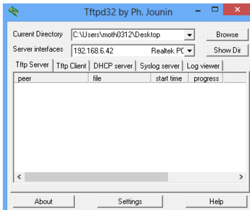
Figure 11-9 Configure Tftpd32
