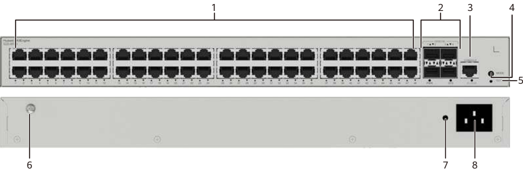
Figure 4-19 S220-48T4X appearance
