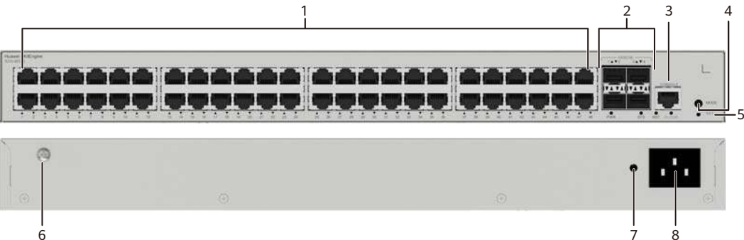
Figure 4-39 S310-48T4X appearance
