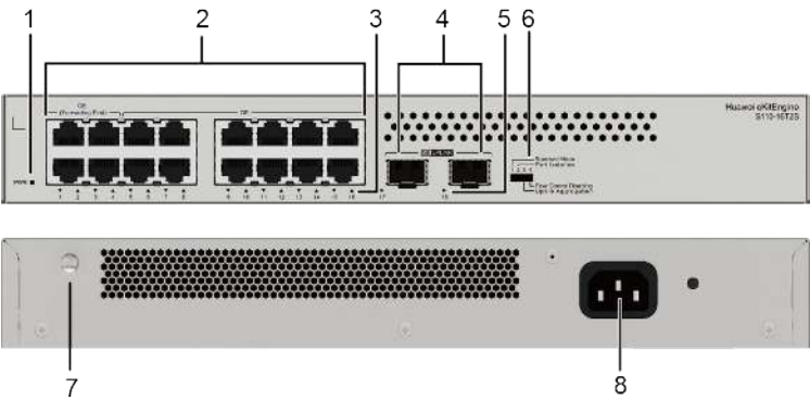
Figure 4-5 S110-16T2S appearance
