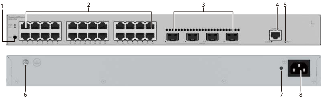
Figure 4-13 S220-24T4X appearance
