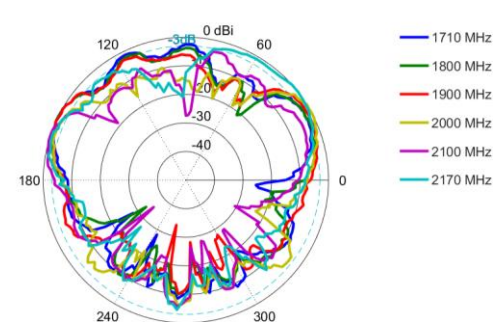
Elevation 1: 1710 – 2170 MHz
