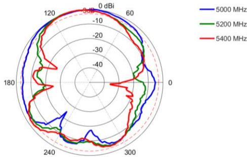
Elevation 2: 5000 – 5400 MHz
