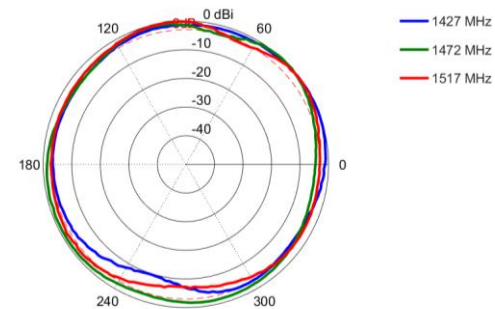
Elevation 2: 1427 – 1517 MHz
