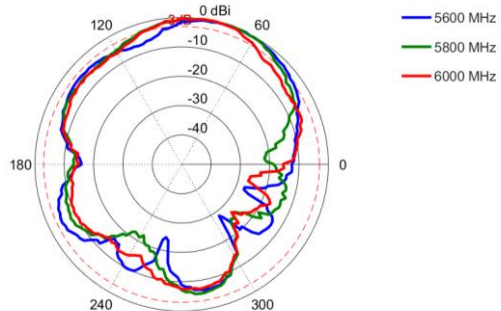
Elevation 2: 5600 – 6000 MHz
