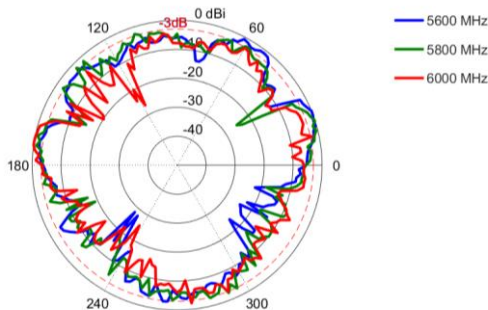
Elevation 1: 5600 – 6000 MHz
