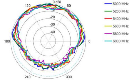
Elevation: 5000 – 6000 MHz
