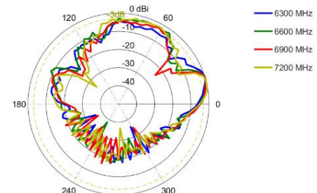
Elevation: 6300 – 7200 MHz
