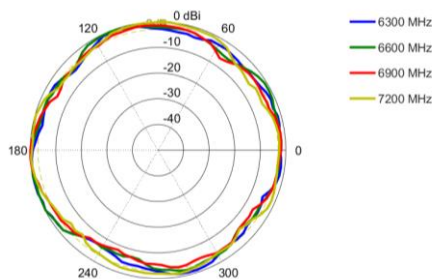
Azimuth: 6300 – 7200 MHz
