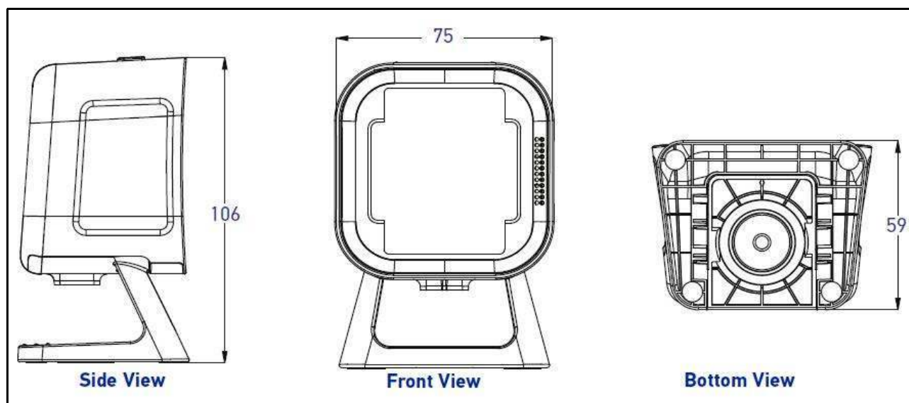
Figure 6. Riser Stand Dimensions
