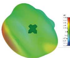
3D Pattern Element 1 (2000MHz)
