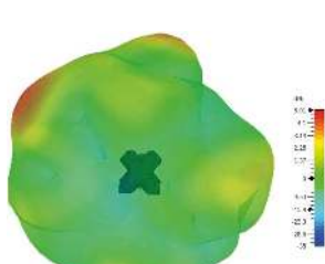
3D Pattern Element 4 (3600MHz)
