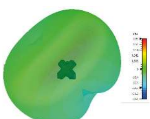
3D Pattern Element 4 (850MHz)
