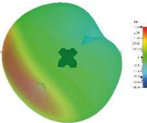
3D Pattern Element 1 (850MHz)
