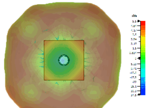
Typical 3D Pattern LTE Elements Top 2600MHz
