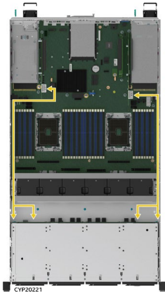
2U Server System Cable Routing
