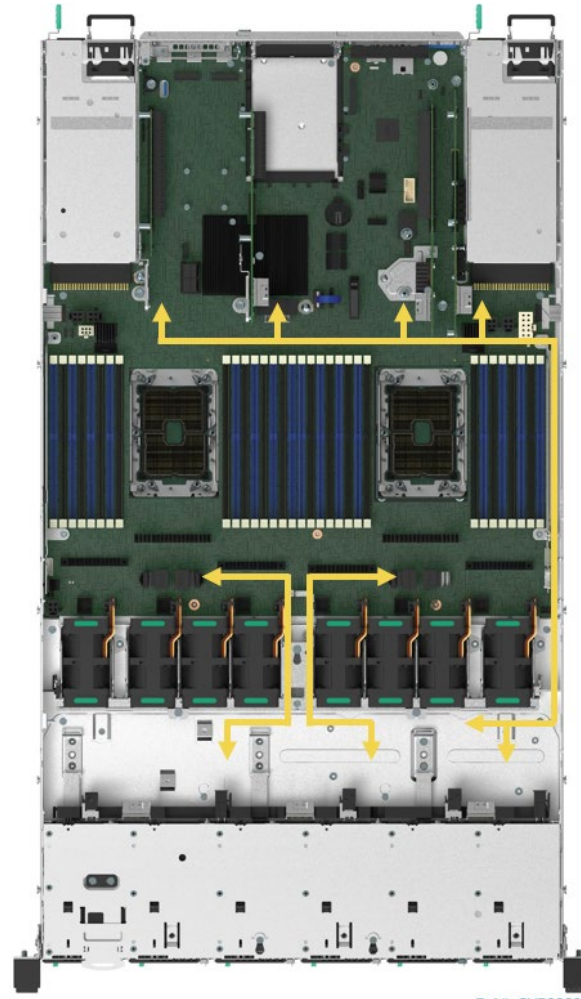
1U Server System Cable Routing
