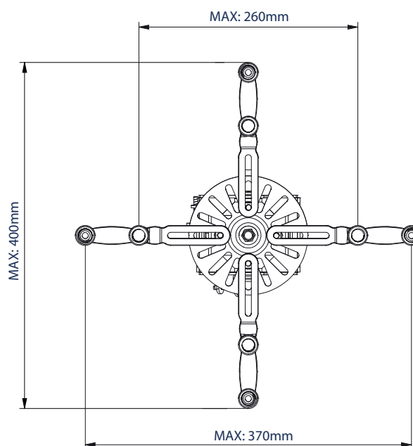
BOTTOM VIEW / INTERFACE
