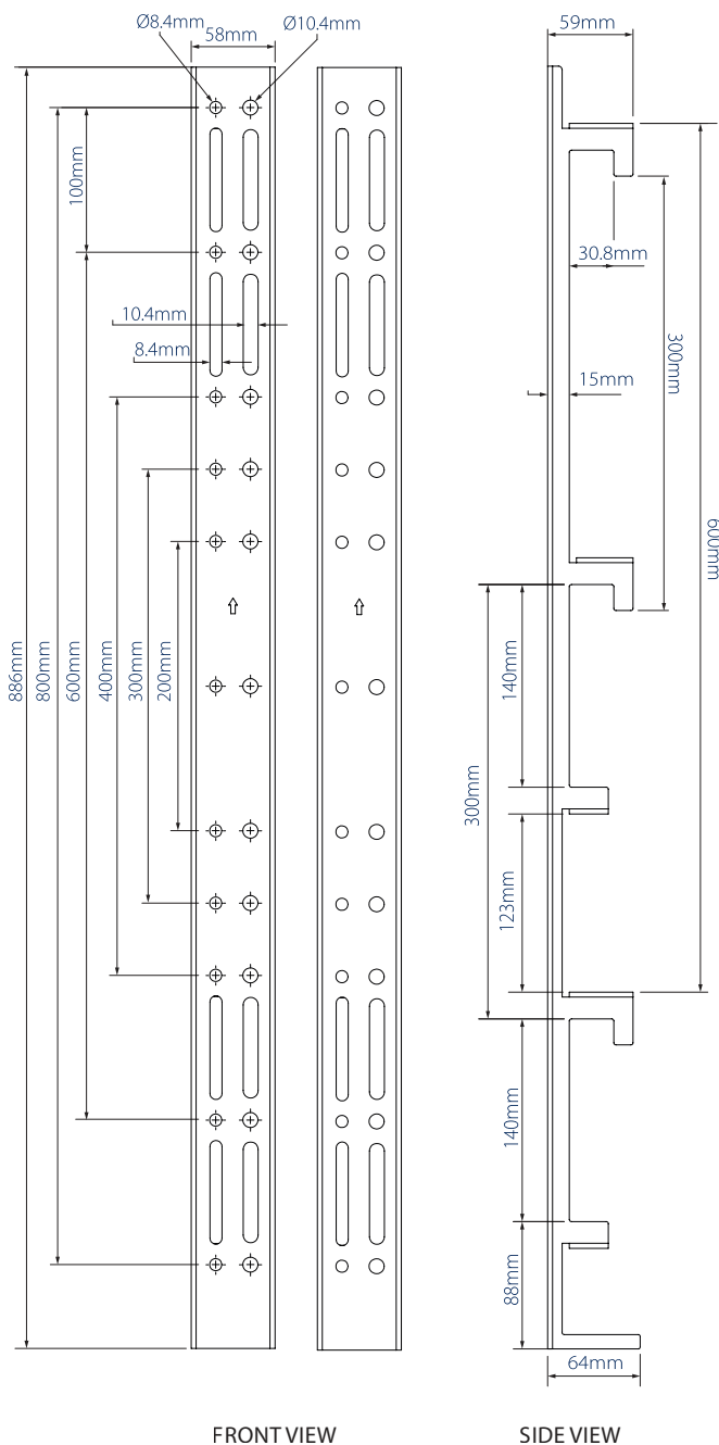
FRONT VIEW
