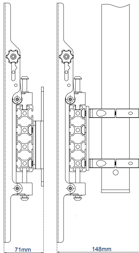
WALL MOUNTED*
