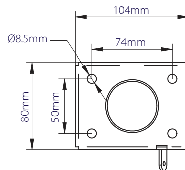
CEILING PLATE
