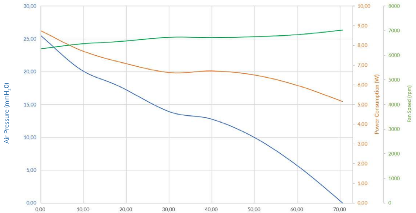
P/Q Curve
