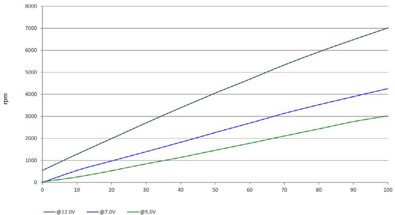
PWM to rpm Curve
