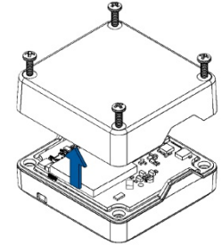
Figure 6 Cover removal
