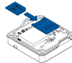
Figure 4 Micro-SIM card insert
