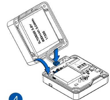
Figure 3 Battery connection
