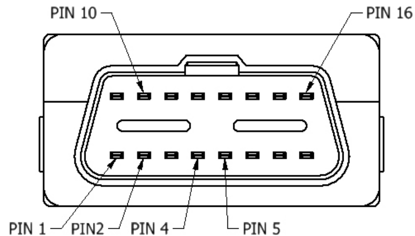
Figure 2 FMB010 OBDII socket pinout
