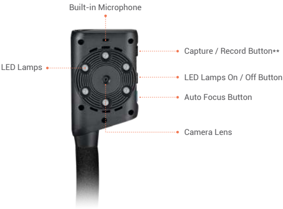
Camera Head
