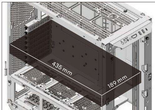
GPU clearance
