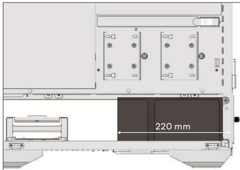
PSU clearance
