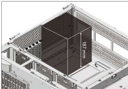
GPU clearance
