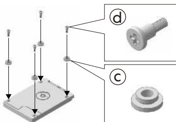
2.5" SSD Installation
