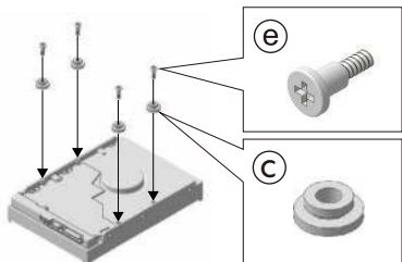
3.5" HDD Installation
