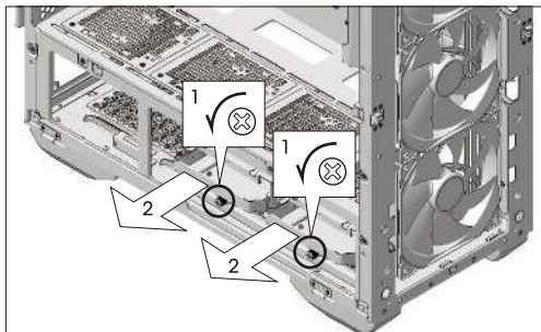
2.5" SSD Installation
