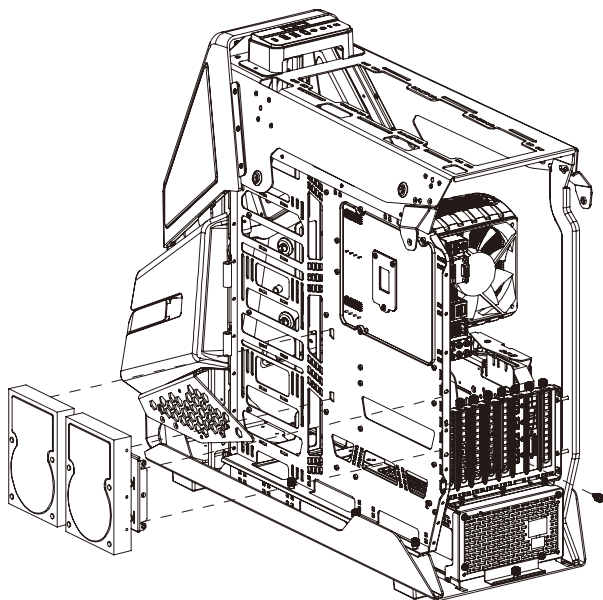
Type A: HDD Installation (With 3.5" HDD Bracket)
