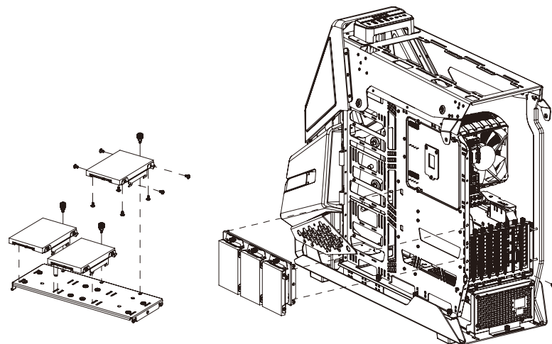
Type C: 2.5" HDD Installation (With 2.5" HDD Bracket)
