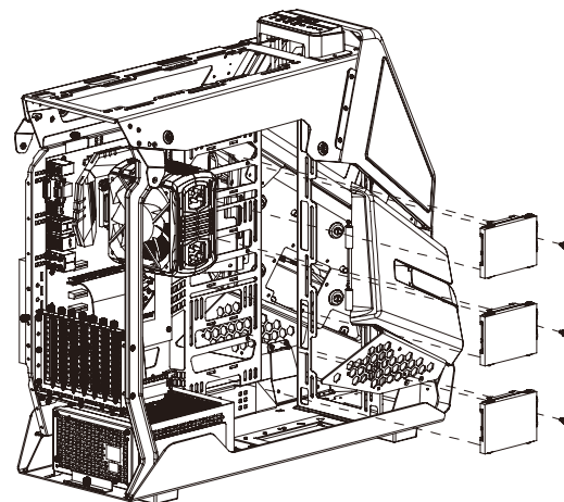
Type C: 2.5" HDD Installation (With 2.5" HDD Bracket)
