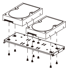
2 x 3.5" HDD
