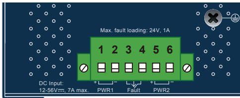
Figure 3-3: Industrial PoE+ Switch Upper Panel
