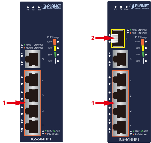
Figure 3-1: IGS-504HPT Front View
