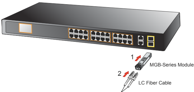
Figure 3-4: Plug In the SFP Transceiver
