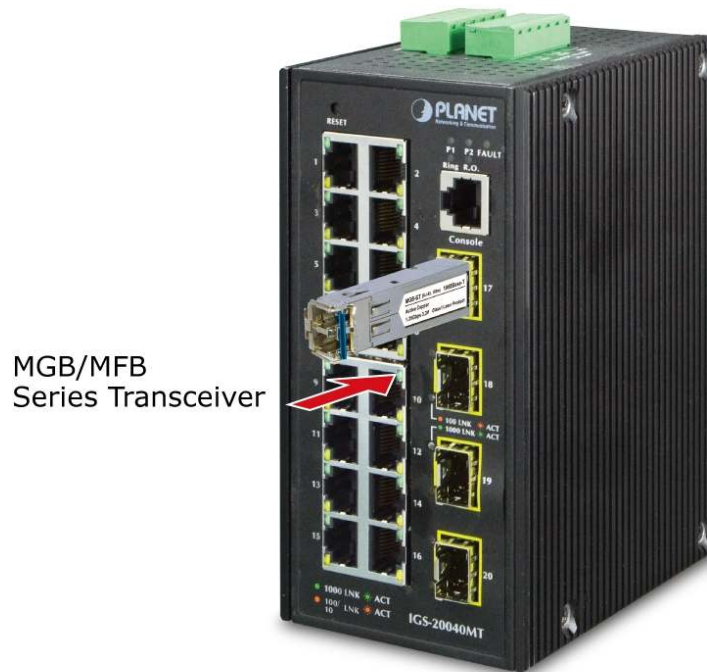
Figure 2-11: Plug in the SFP/SFP+ Transceiver
