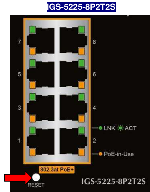
Figure 2-4: IGS-5225-8P2T2S Reset Button
