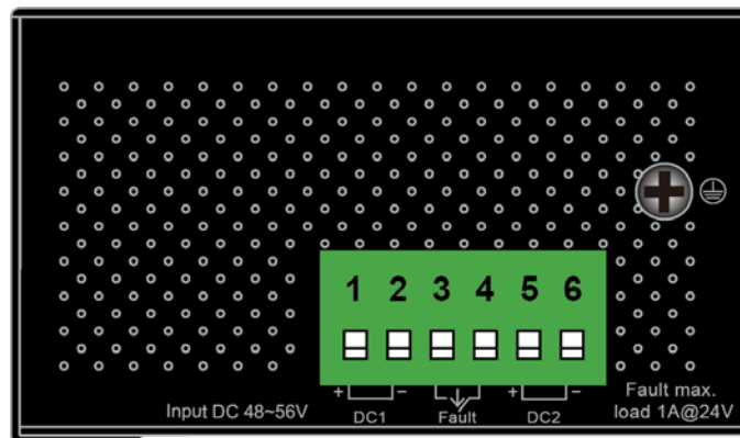
Figure 2-7: IGS-5225-4P2S Upper Panel
