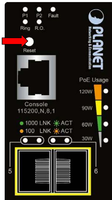
Figure 2-5 IGS-5225-4P2S Reset Button
