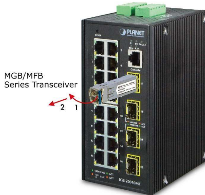
Figure 2-12: Pull out the SFP/SFP+ Transceiver Module
