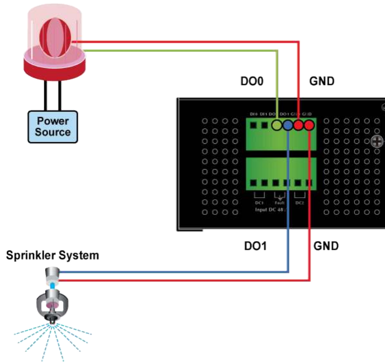
Figure 2-10 Wires DO0 and DO1 to Open Detector
