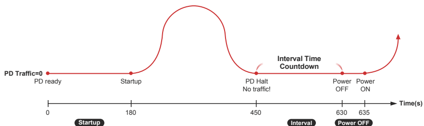
Figure 2-4: Alive Check Mechanism
