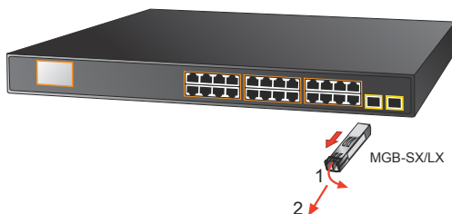
Figure 3-5: How to Pull Out the SFP Transceiver
