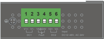
Figure 2-2: IXT-705AT Upper Panel
