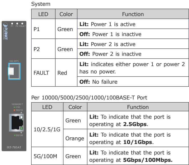
Figure 2-1: IXT-705AT Front Panel
