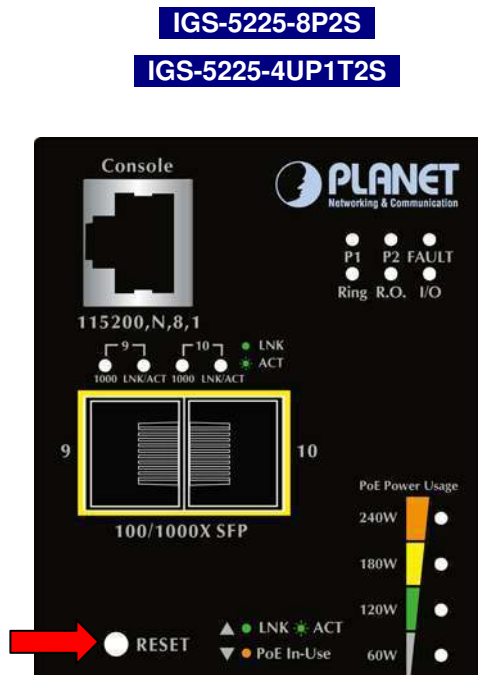
Figure 2-8: IGS-5225-8P2S/IGS-5225-4UP1T2S Reset Button
