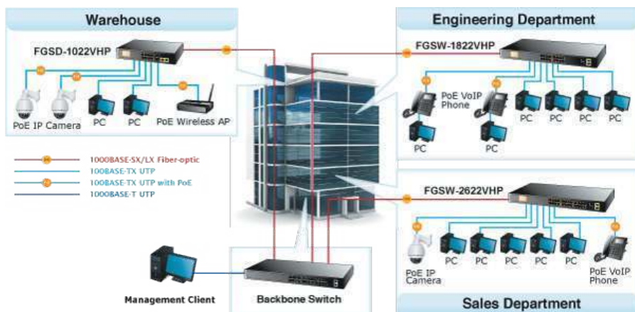
Figure 3-6: Department/Workgroup 802.3at PoE+ Switch Connection
