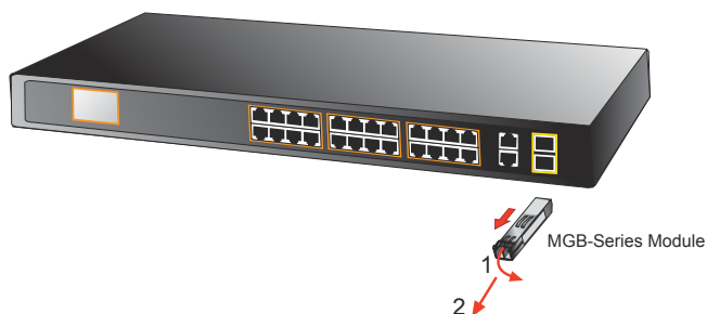
Figure 3-5: How to Pull Out the SFP Transceiver
