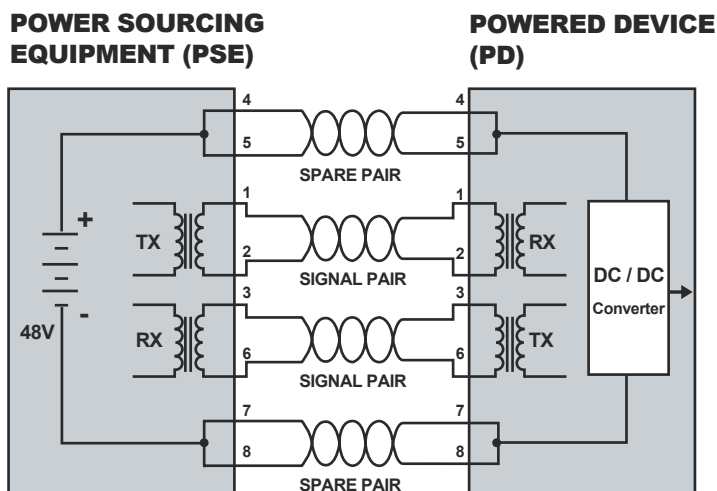
Figure 1: Power Supplied over Spare Pins
