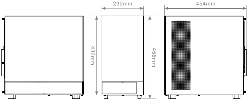
Chassis dimension
