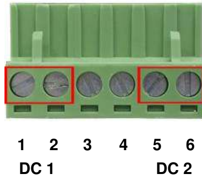
Figure 2-18 6-Pin Terminal Block Power Wiring Input
