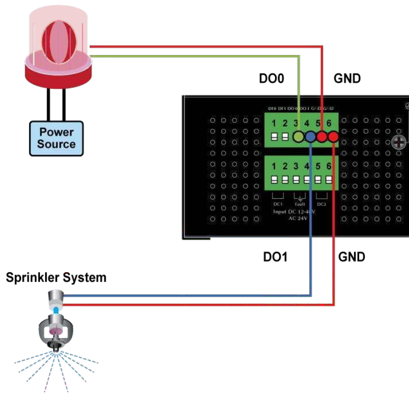
Figure 2-22 Wires DO0 and DO1 to Open Detector
