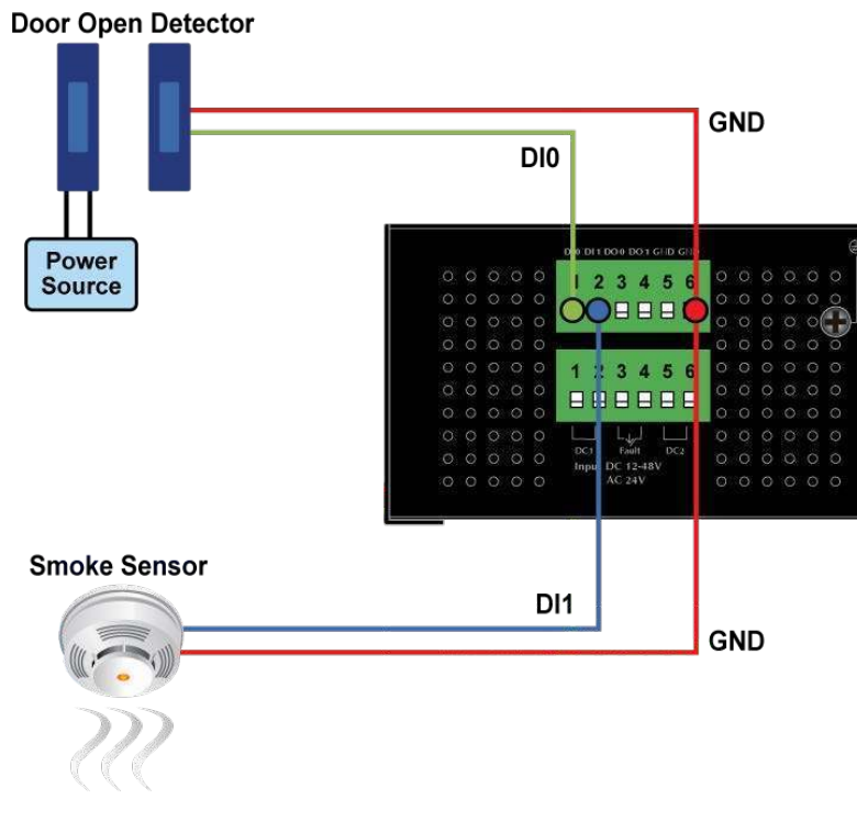
Figure 2-21 Wires DI0 and DI1 to Open Detector
