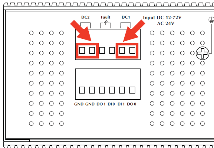
Figure 2-16: IGS-12040MT Upper Panel
