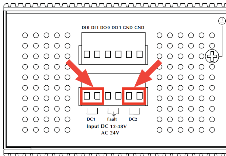
Figure 2-17: IGS-20040MT Upper Panel
