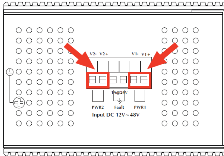
Figure 2-15: IGS-10080MFT Upper Panel
