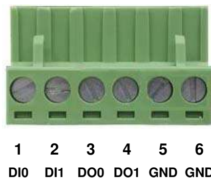
Figure 2-20 6-Pin Terminal Block DI / DO Wiring Input
