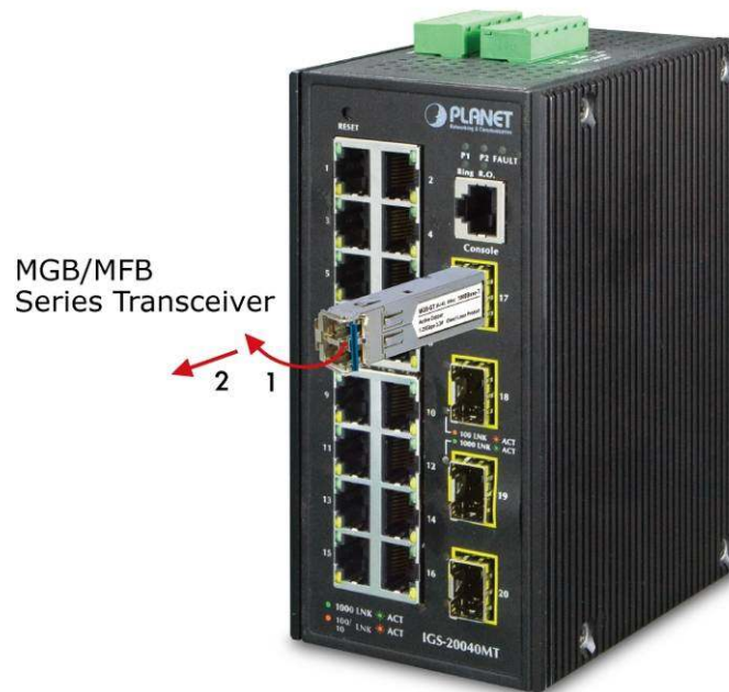
Figure 2-10: Pull out the SFP Transceiver Module
