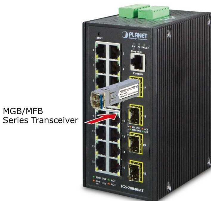
Figure 2-23: Plug-in the SFP Transceiver
