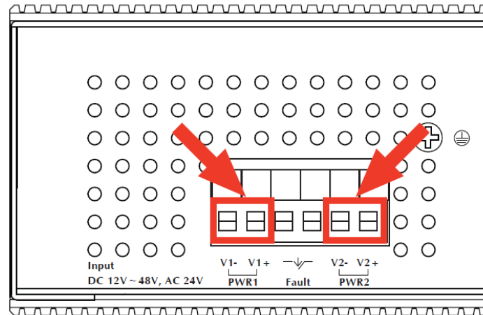
Figure 2-13: IGS-10020MT Upper Panel
