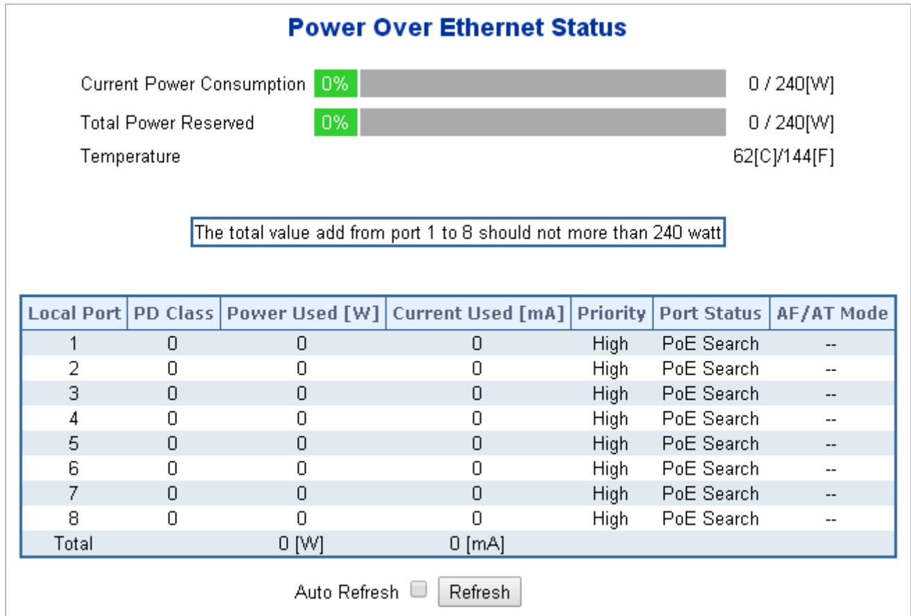
Figure 4-16-5: PoE Status Screenshot
