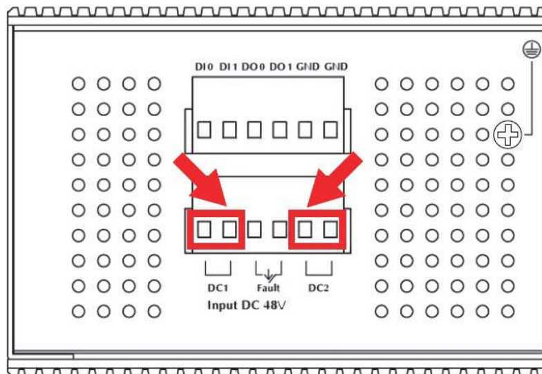
Figure 2-14: IGS-10020PT/HPT Upper Panel
