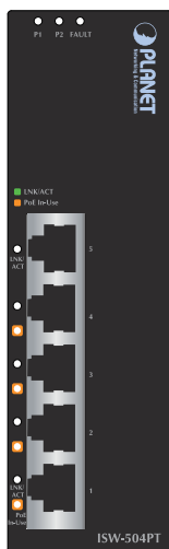
Figure 2-1 ISW-504PT front panel
