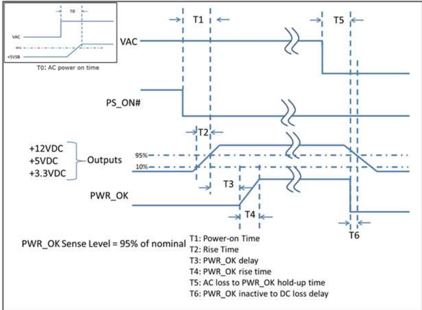
Figure 1 Time Diagram
