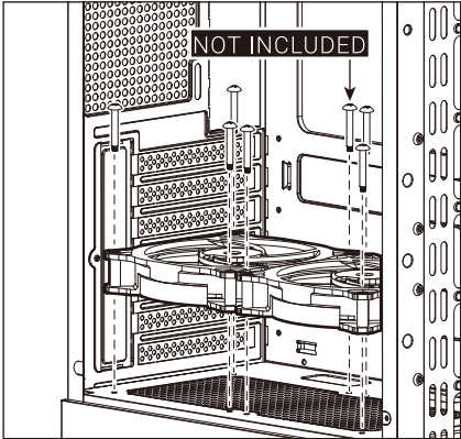
(7d) Install PSU Fans
