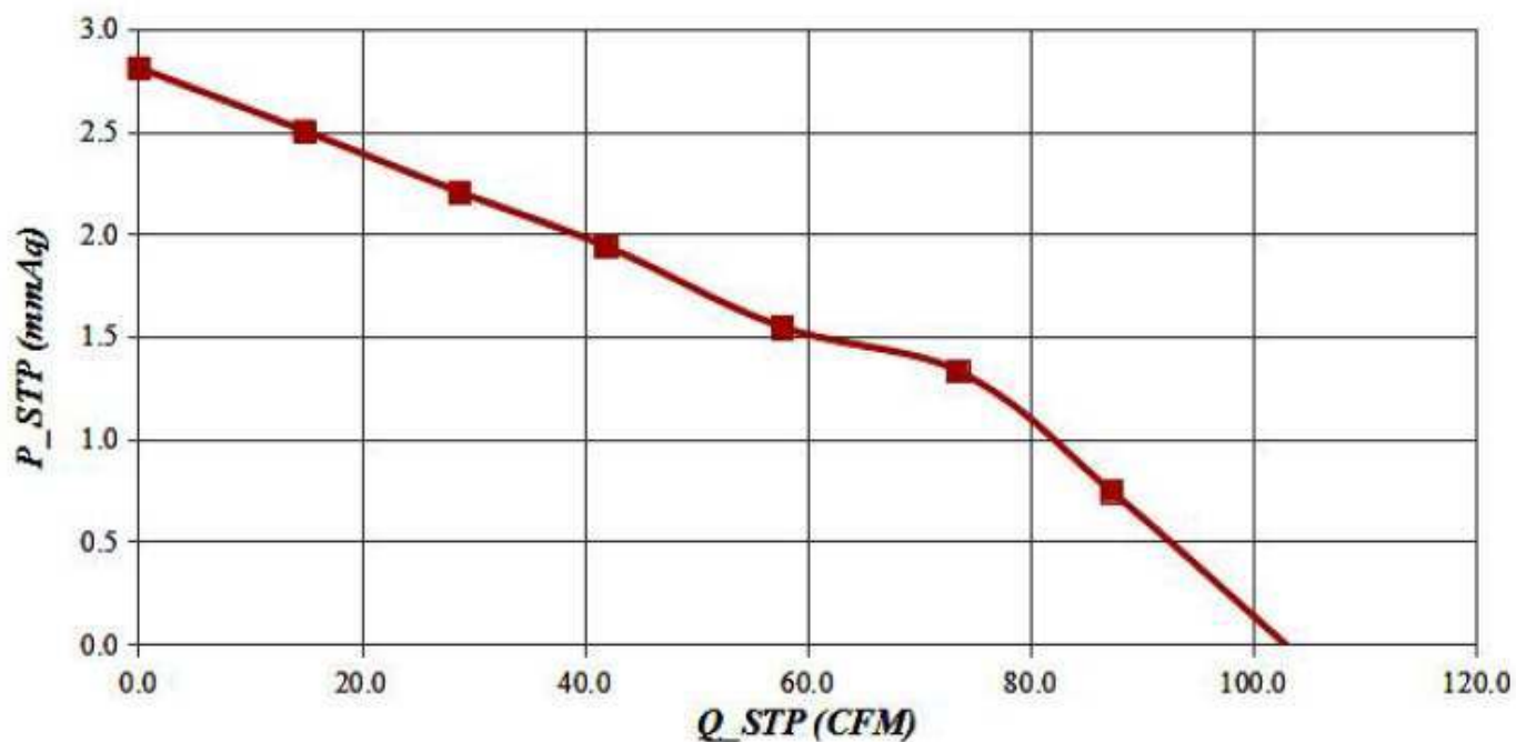
P-Q Curve
