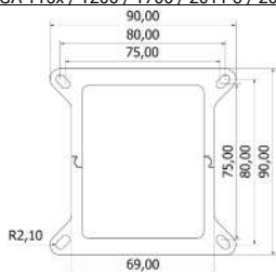
LGA 3647 Square
