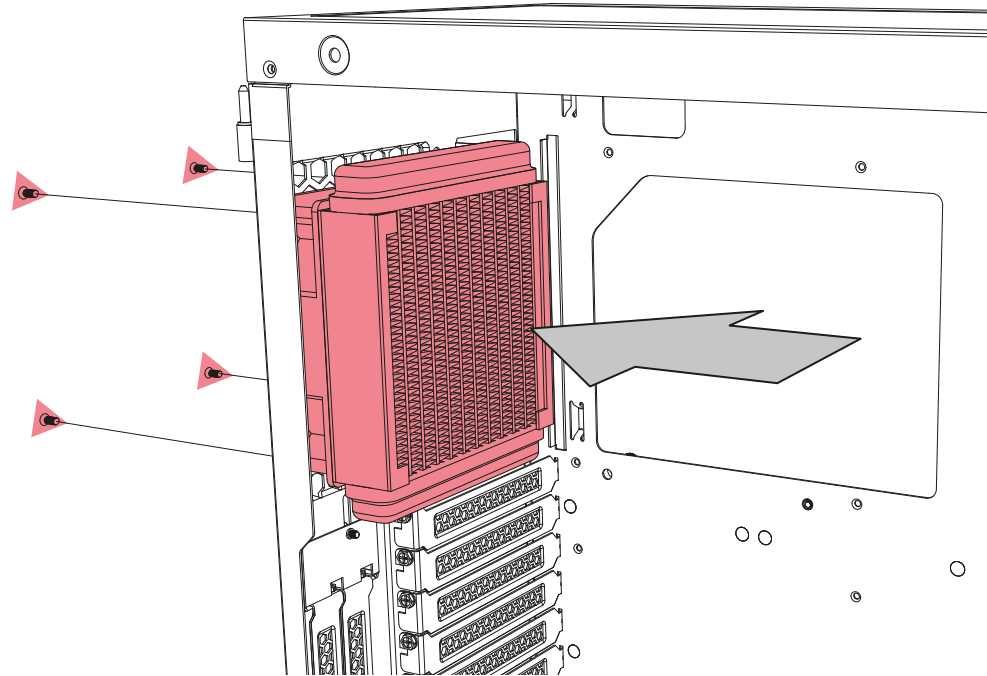
120 mm Radiator
